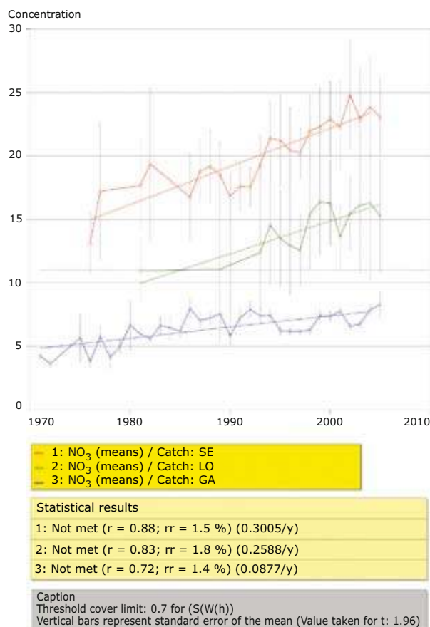
Figure 36 Nitrate trends at basin level: Seine, Loire, Garonne (left: all data, right: Eionet data set)
