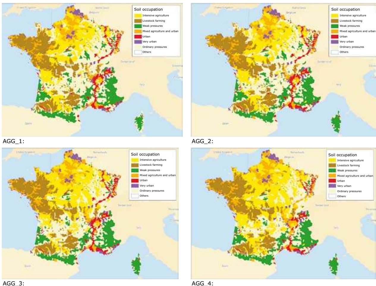
Figure 40 Example of catchment distribution related to small changes I scenario codification
